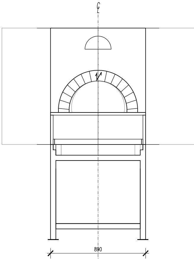
MODEL OT 180 FRONT VIEW
