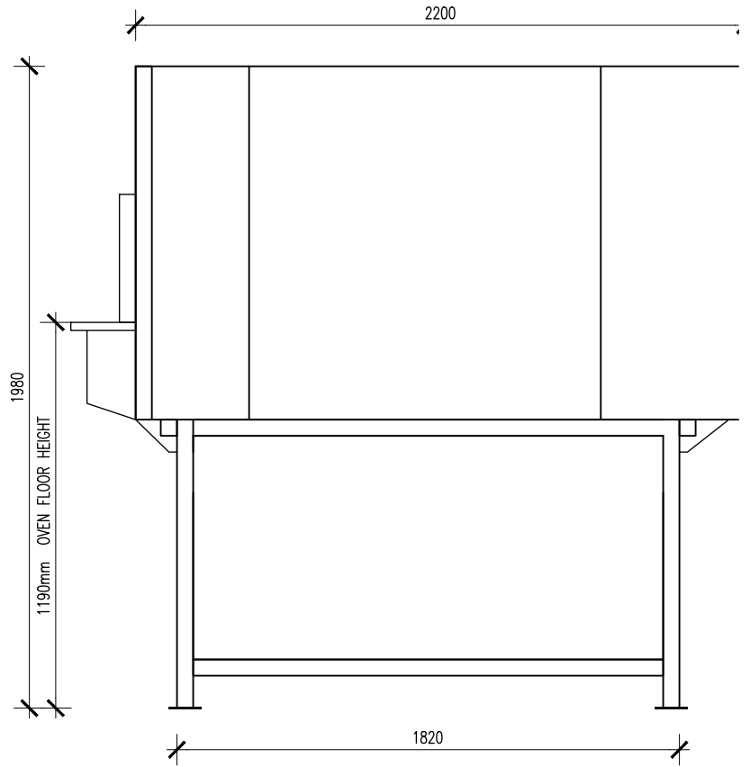
MODEL OT 180 SIDE VIEW
