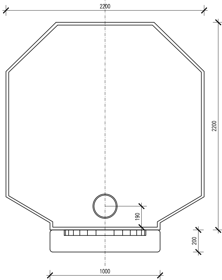
MODEL OT 180 PLAN VIEW
