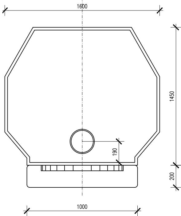
MODEL OT 120 PLAN VIEW
