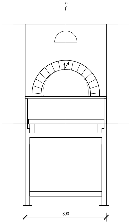
MODEL OT 120 FRONT VIEW
