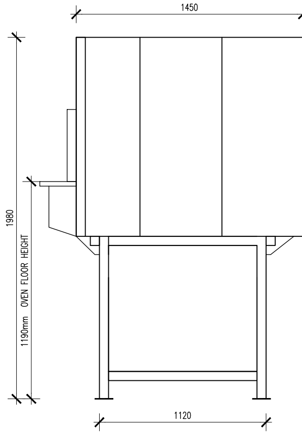
MODEL OT 120 SIDE VIEW
