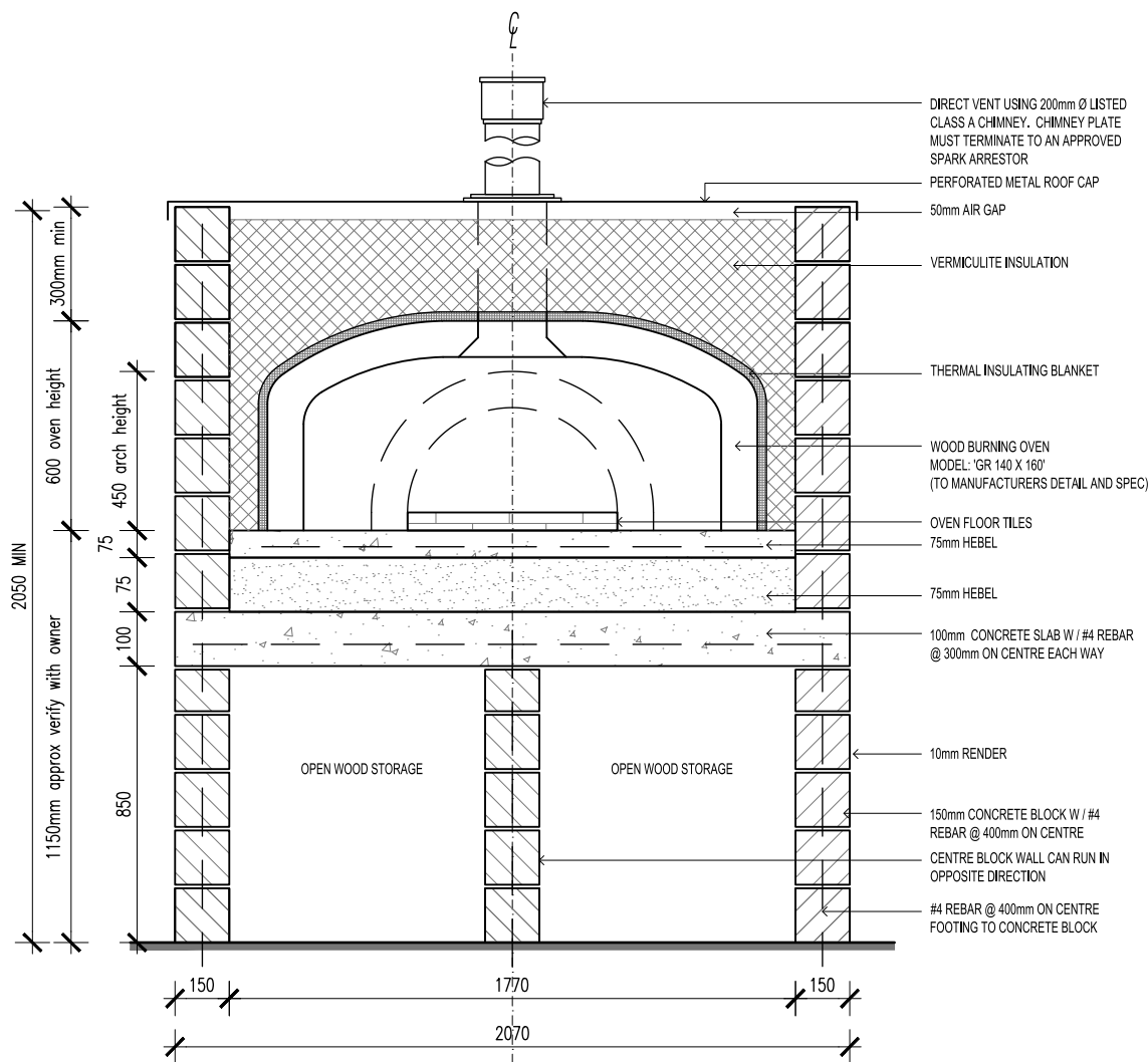
MODEL GR140 X 160 FRONT VIEW
