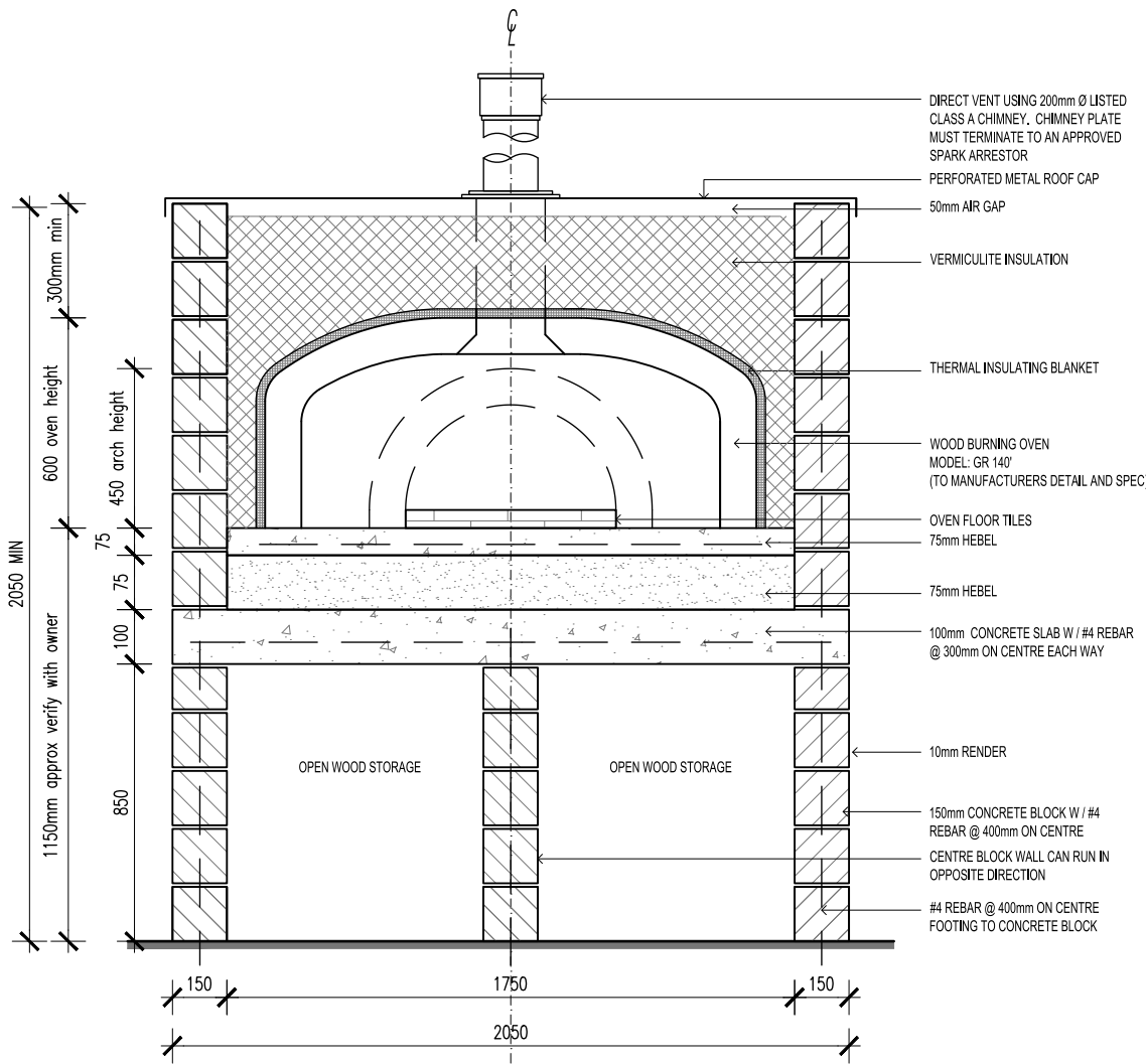
MODEL GR140 FRONT VIEW
