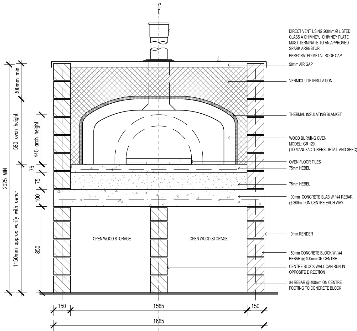
MODEL GR120 FRONT VIEW
